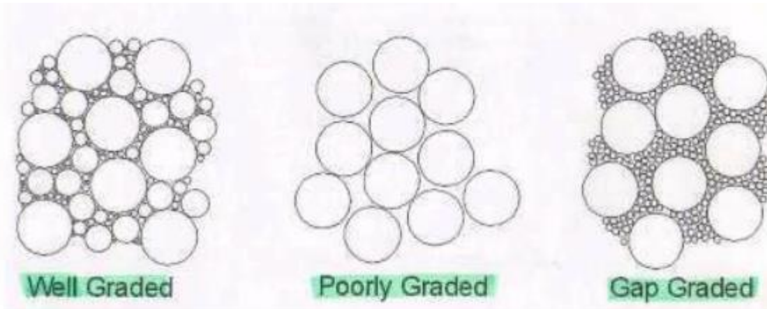
Fig.7: aggregate grading types
