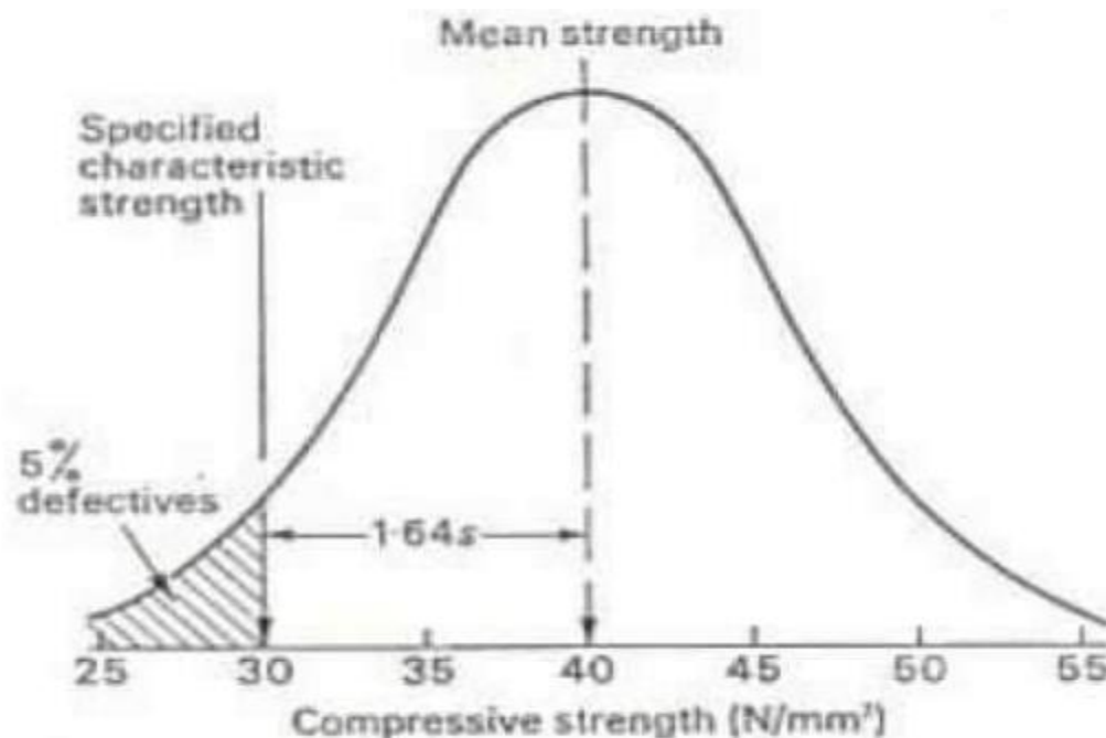
Fig.1: Means compressive strength vs characteristic compressive strength
